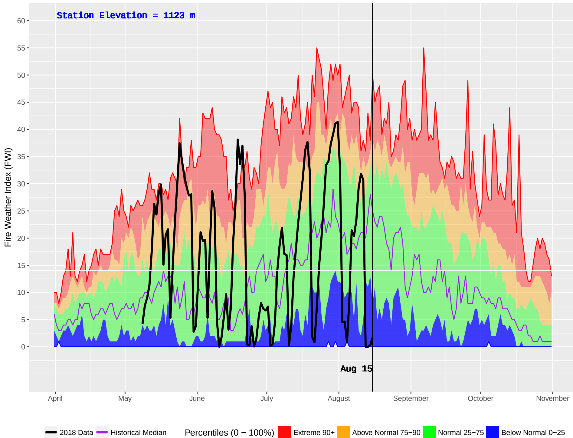
MCLEAN LAKE (311) : Historical (1987–2016) and Current (2018) Daily Fire Weather Index (FWI)
