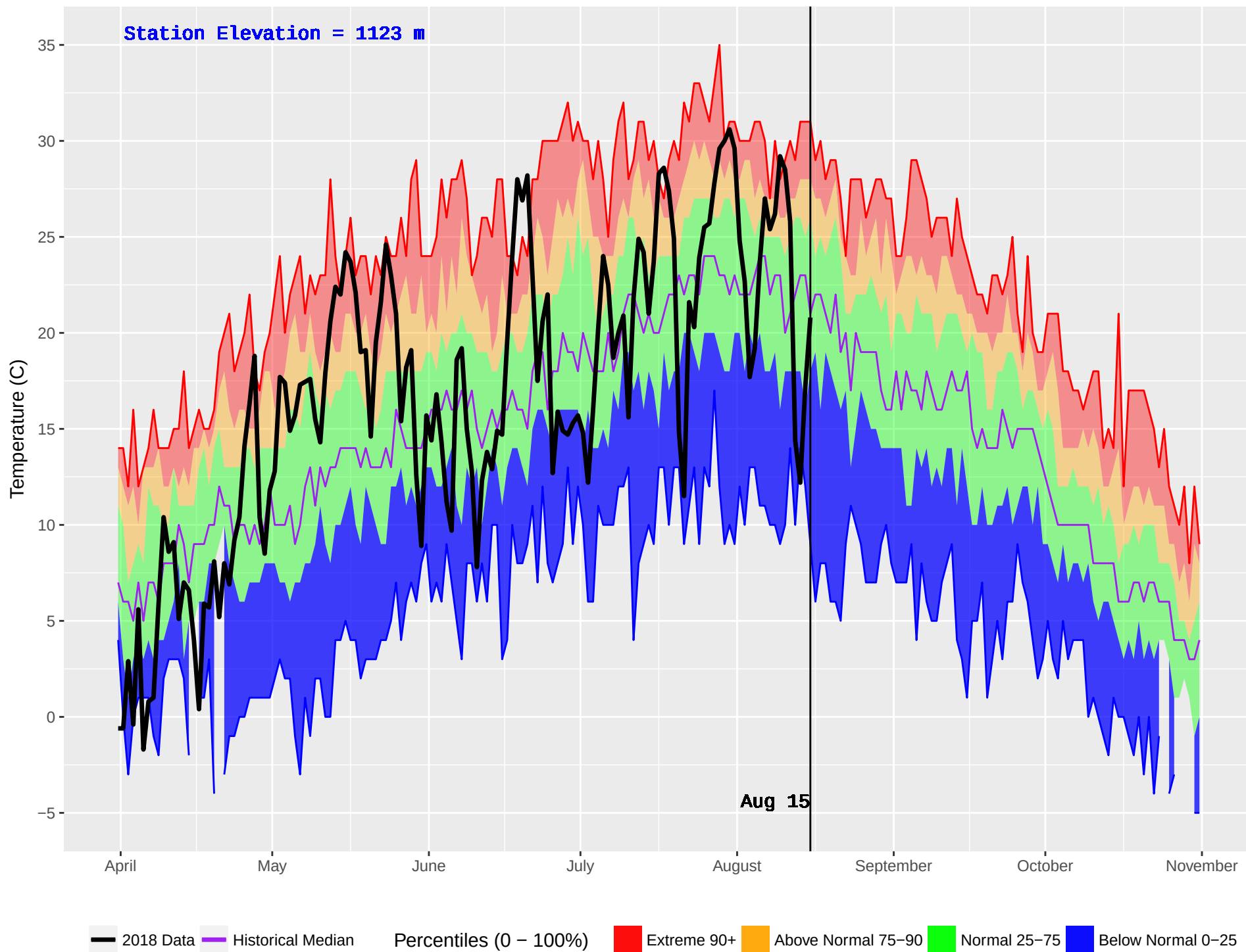
MCLEAN LAKE (311) : Historical (1987–2016) and Current (2018) Daily Temperature
